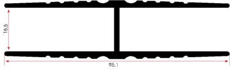
FSM 706 1,400 kg/m
